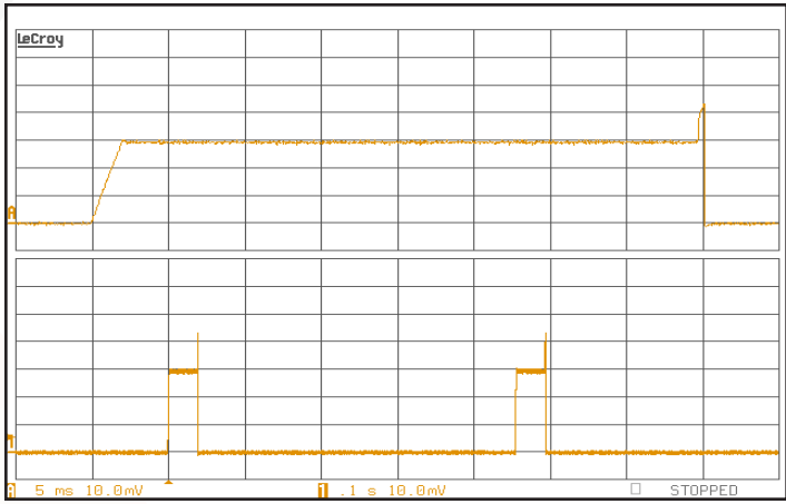
Figure 18: Load current (5 A/div) as a function of time (5ms/div and 100ms/div) when the converter attempts to turn on into a 10 m\Omega short circuit.
