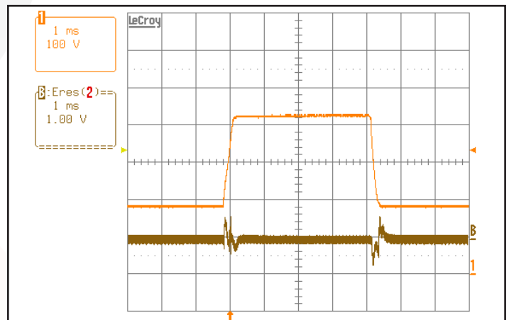
Figure 12: Output voltage response to step-change in input voltage (250V/ms). Load cap: 1 \mu F ceramic capacitor and 10 \mu F tantalum capacitor. Ch 1: V_{in} (100 V/div), Ch 2: V_{out} (1 V/div).
