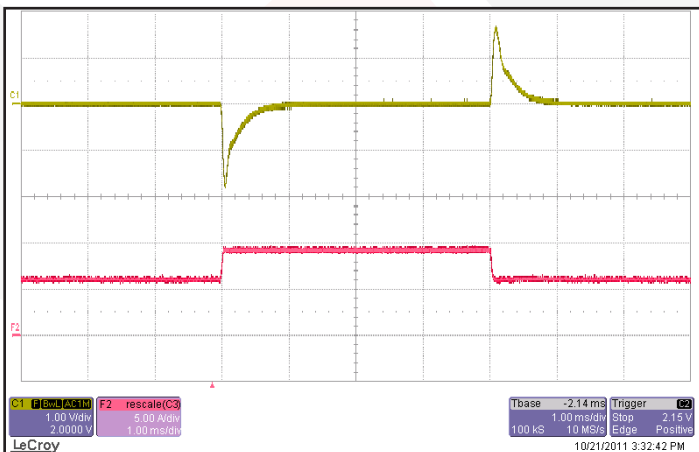
Figure 11: Output voltage response to step-change in load current (50%-75%-50% of I_{out(max)} ; di/dt = 0.1 A/\mu s ). Load cap: 1 \mu F ceramic capacitor and 10 \mu F tantalum capacitor. Ch 1: V_{out} (1 V/div), Ch 2: I_{out} (5 A/div).
